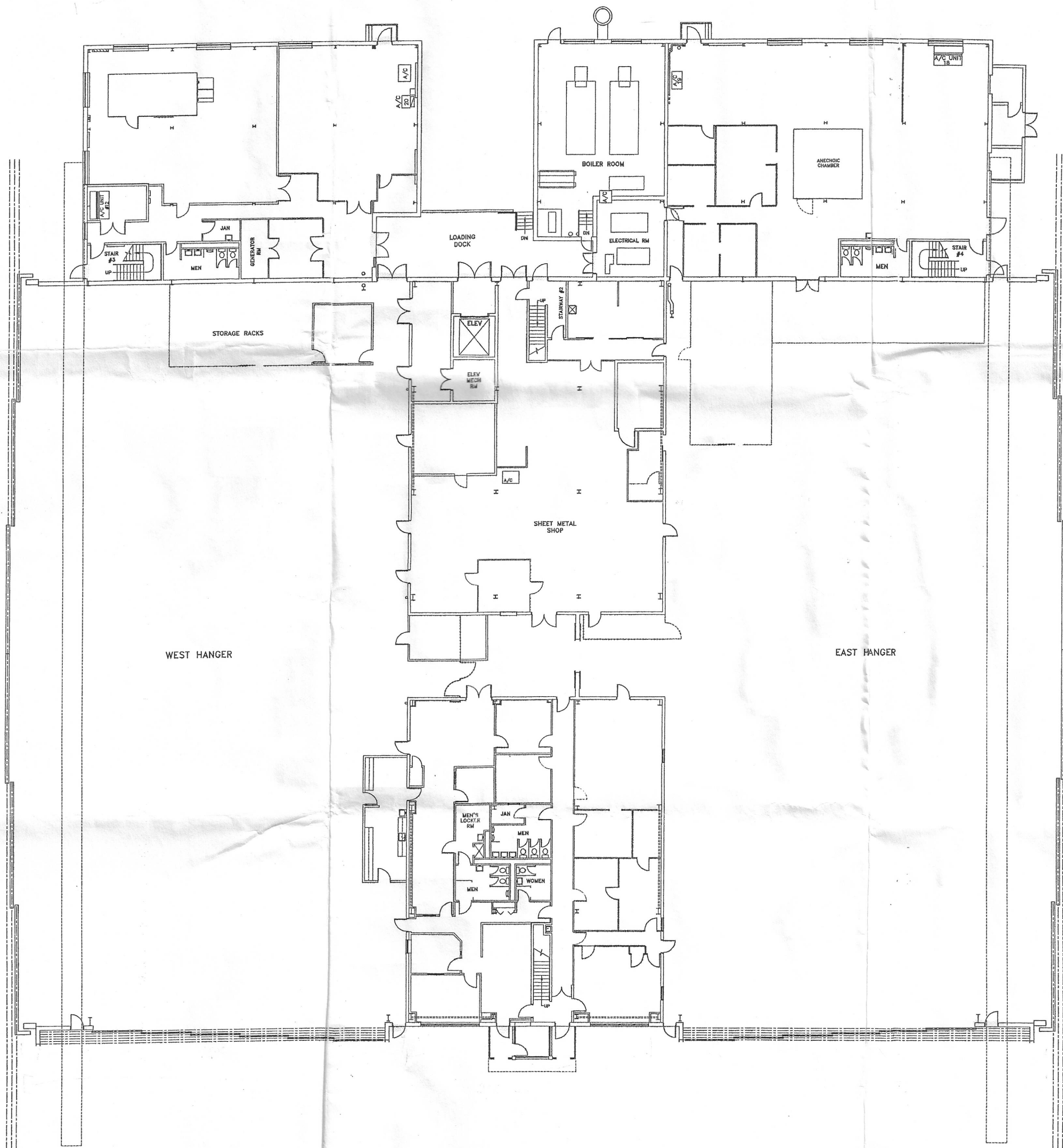
FIRST FLOOR 1/16"=1'-0"
