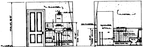
BATH ROOM ELEVATIONS SCALE 1/8" = 1'-0"
