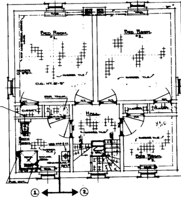
SECOND FLOOR PLAN SCALE 1/4" = 1'-0"
